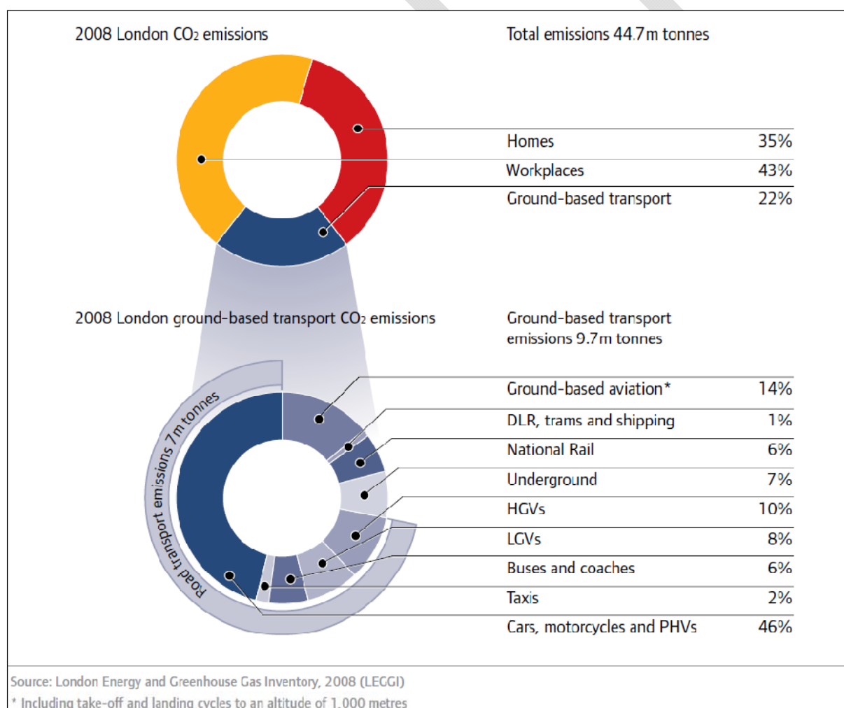
Figure 21: Transport's contribution to London's CO 2 emissions 25
